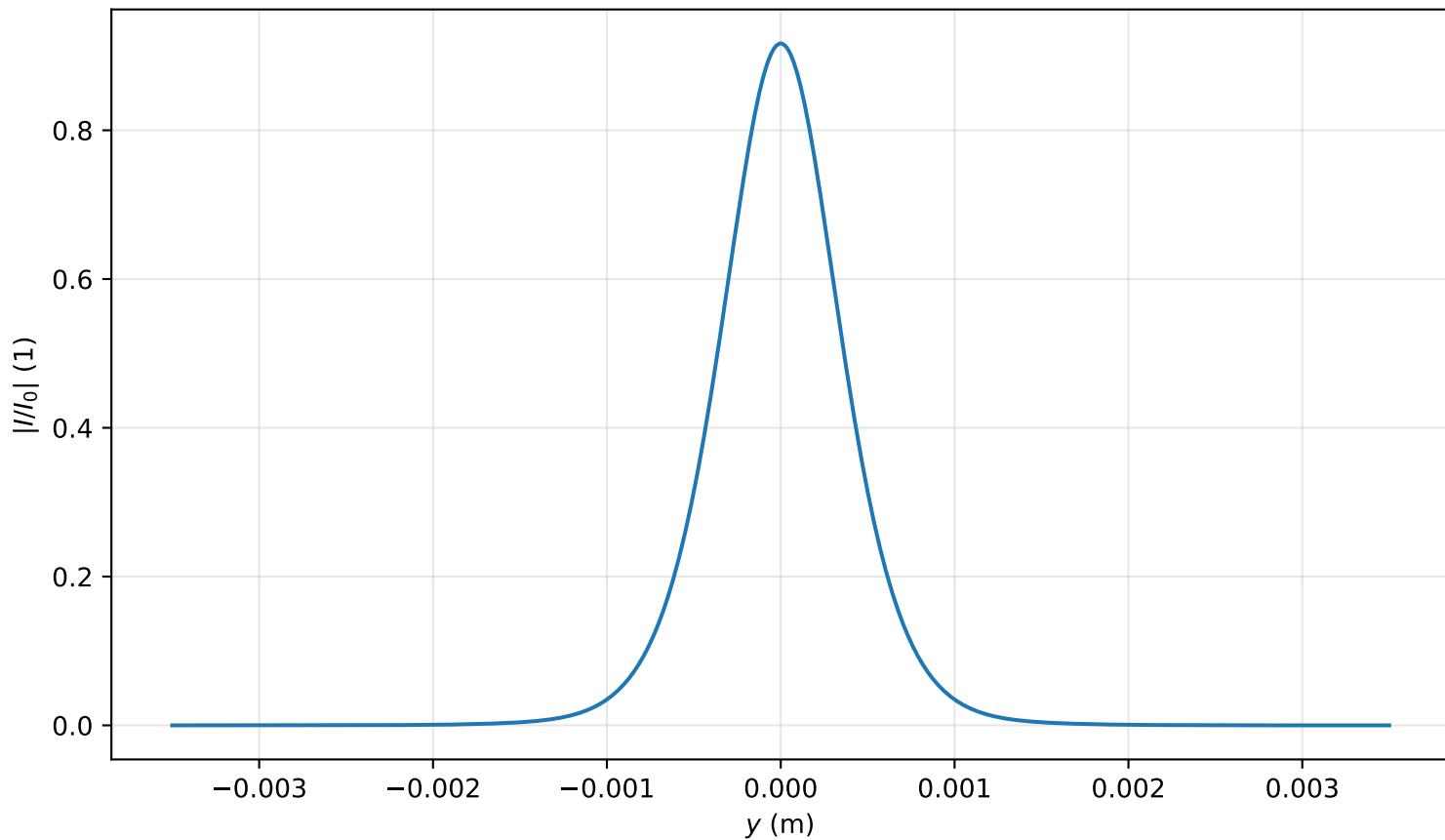
Intensity profile I(x=0, y, z=2.707)/I_0 , P_{in}=0.7P_{cr} , artificial time
